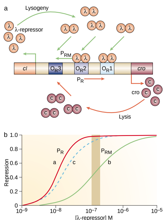
Figure 2 | Modelling the \lambda -bacteriophage circuitry.
